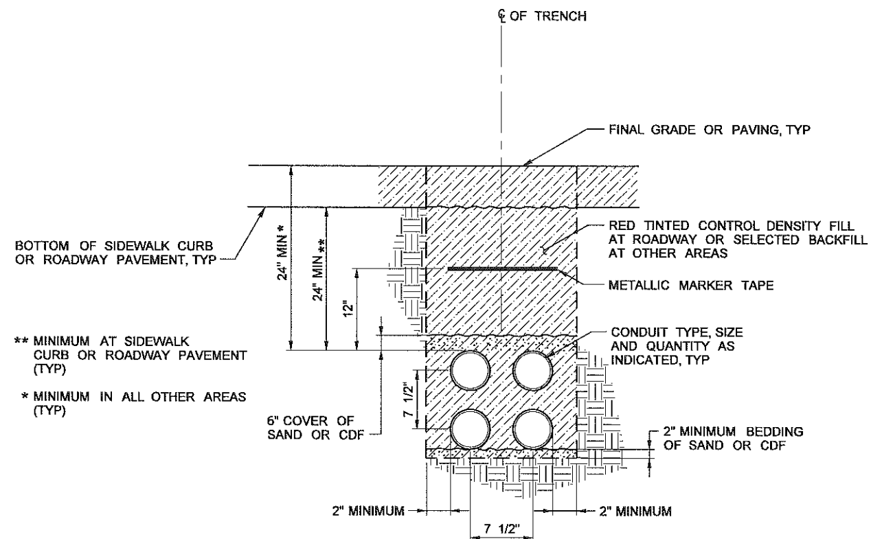
TRENCHED UNDERGROUND 600 V CONDUIT - TYPICAL 2
