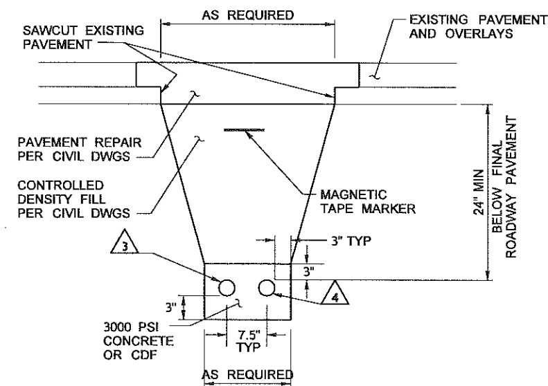
TRENCHED UNDERGROUND 600 V CONDUIT - TYPICAL 2
